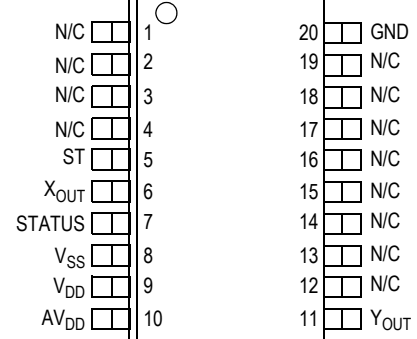
Figure 2. Pin Connections
